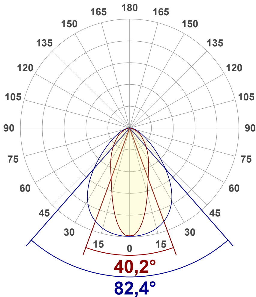
Luminous Intensity diagram Unit: 0-100% of peak intensity
